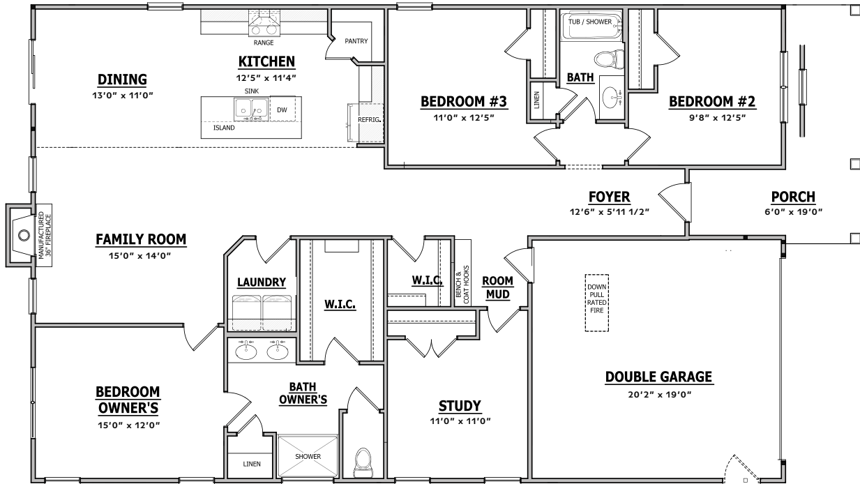
FIRST FLOOR
