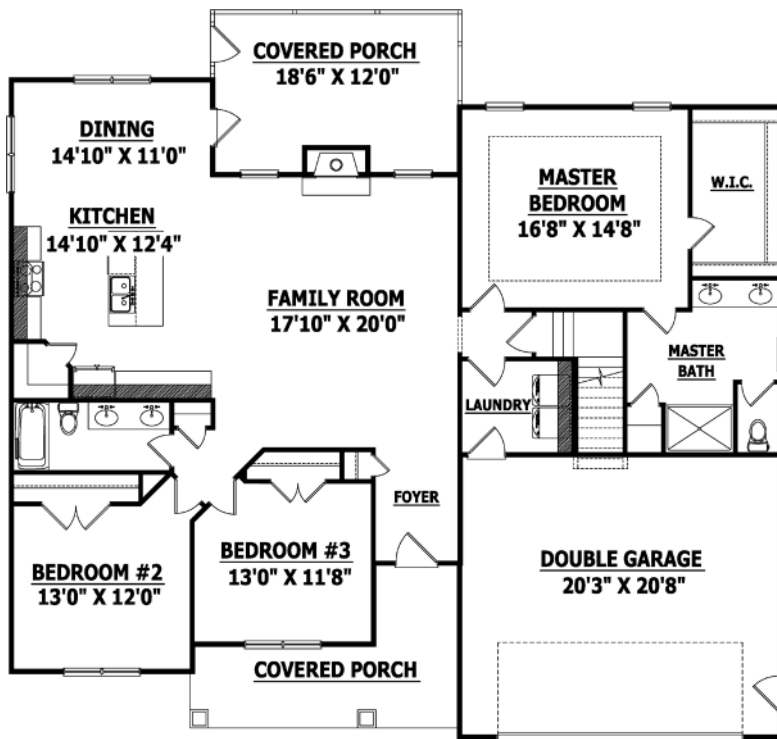
FIRST FLOOR
